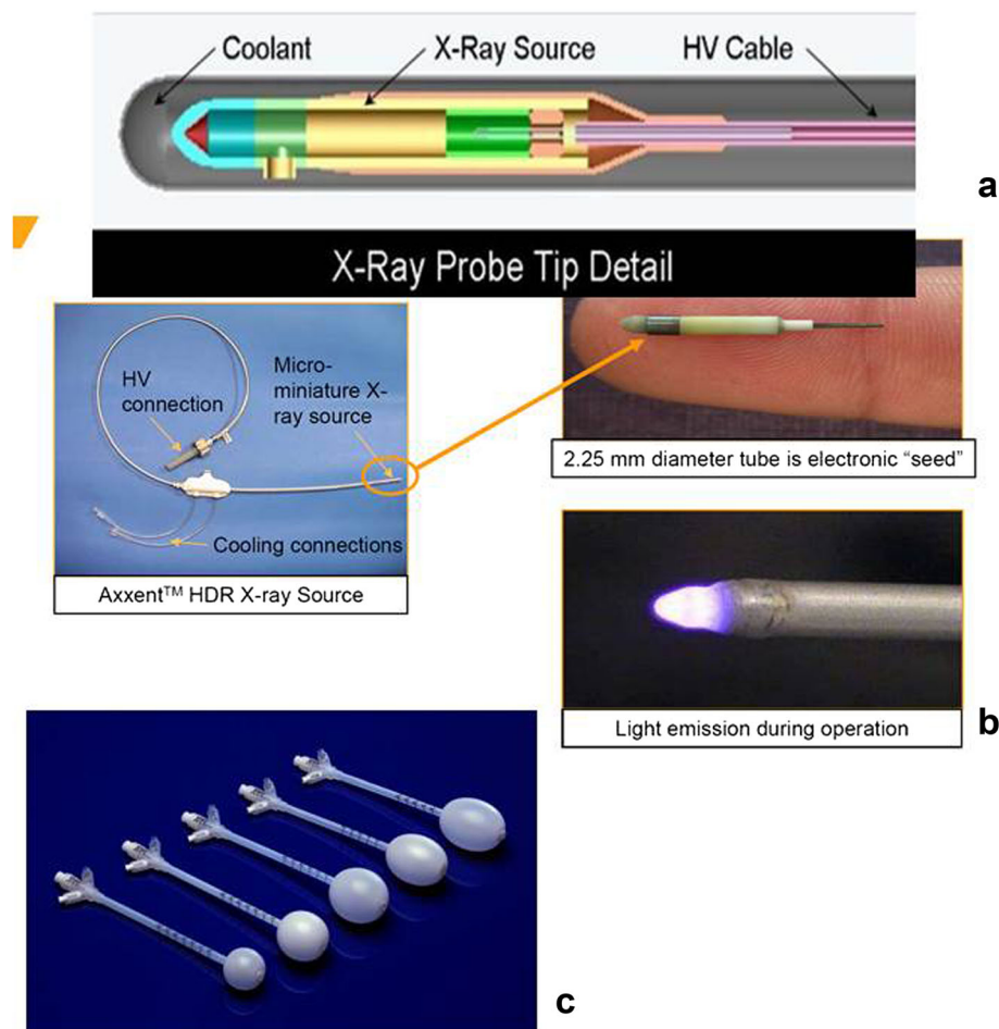
Fig. 5 The Xoft Axxent System (Xoft Inc. 345 Potero Ave. Sunnyvale, CA 94085, USA). a Schematic diagram of the X-ray source. b Left: the cooling tube in which the source is guided to the irradiation position. Right top: The source, bottom: light emission during source operation. c Spherical balloon applicators for breast IORT
