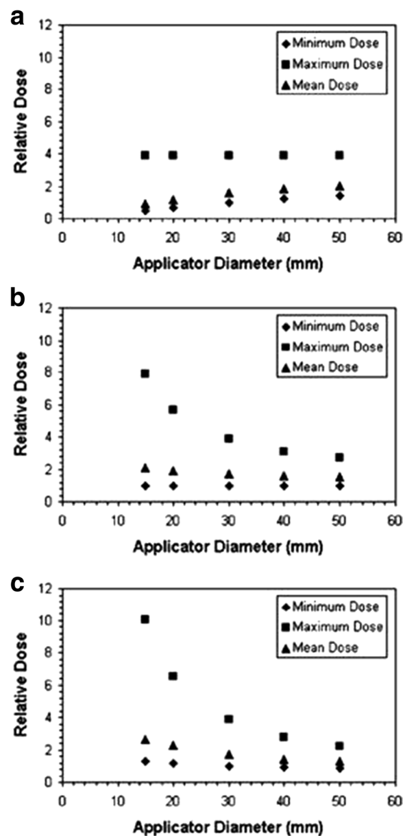
Fig. 6 Maximum, mean and minimum doses in 10 mm thick spherical shells of tissue surrounding Intrabeam breast applicators for different depths of prescription of the reference dose with different sizes of applicators. a prescription at the applicator surface. b prescription at 10mm distance from the applicator surface. c prescription at 20mm distance from the applicator surface. The prescription dose is defined as unity for the minimum target dose with the 30mm applicator in each diagram. For small applicators, a prescription at the applicator surface (a) produces smaller overdoses at the applicator surface, however also lower doses at a depth of 10mm which is considered as the margin surrounding the tumor cavity which must be treated. Prescription at 10mm depth ensures that the desired dose arrives at this depth, produces higher overdoses for small applicators, prescription at 20mm depth increases the overdoses. Therefore the authors conclude that a prescription at 10mm depth is the best compromise in order to ensure that desired dose arrives at depth for all applicator sizes. From Ebert and Carruthers (2003) [35]
