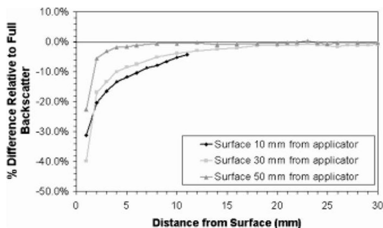
Fig. 7 Dose reduction due to missing backscatter at different depths under the tissue surface for three different depths of the applicator surface in tissue (10mm, 30mm and 50mm) for a 30mm diameter intrabeam applicator. For shallow depths of the applicator dose reduction in superficial tissues can amount as much as 25-40%. From Ebert and Carruthers (2003) [35]
